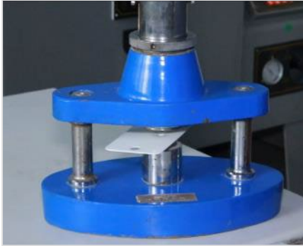
Punching Resistance Test 50cm on both sides
