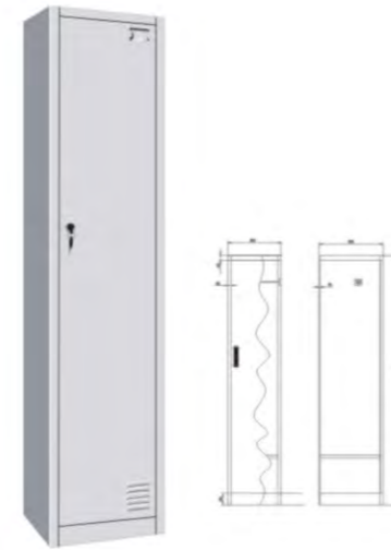
JF-1B1A H1850 × W380 × D450mm
