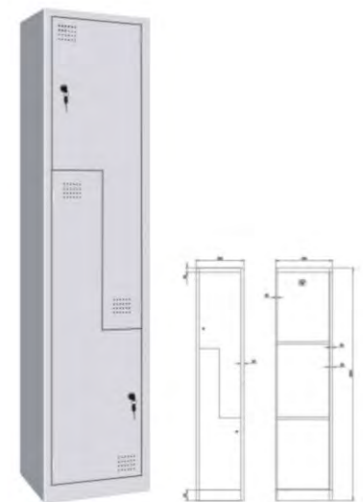
JF-Z001 H1850 × W400 × D450mm
